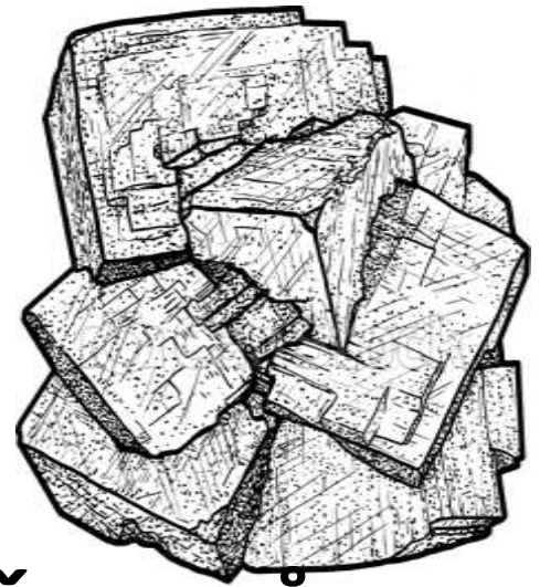
Fluorite
